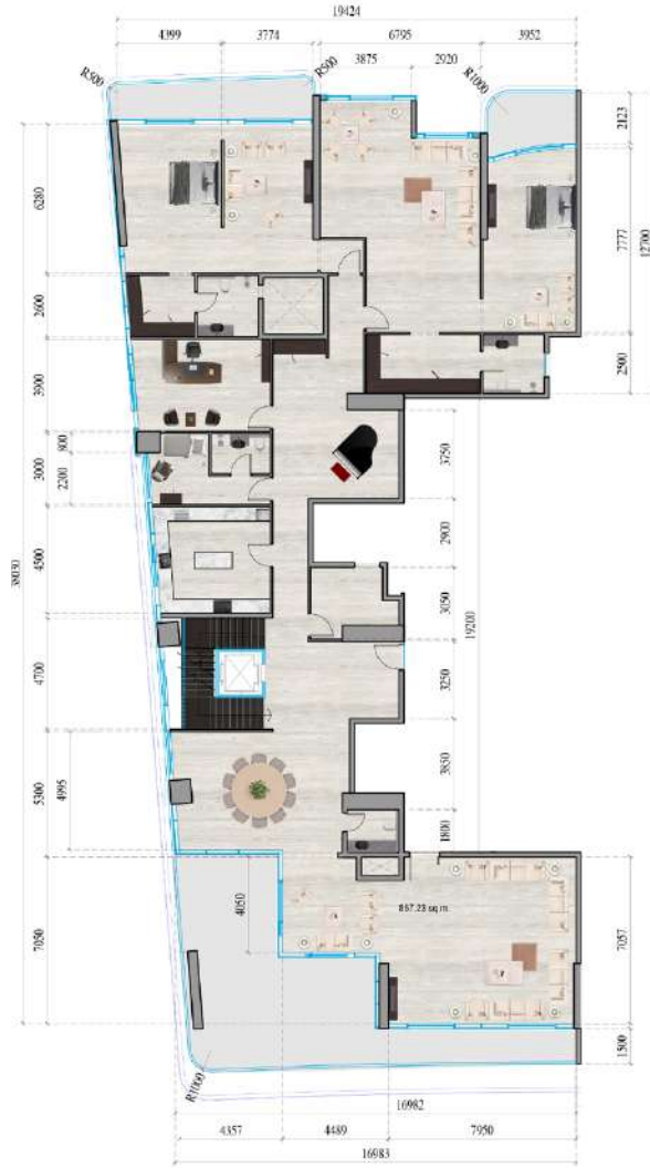
① 45th FLOOR PLAN DUPLEX 2 - LOWER FLOOR
